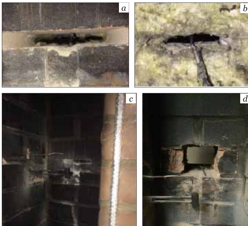
Figure 58a-c. Details of joints used for 'failed mortar' tests. Figure 58d. Detail of joint used for 'failed brickwork' tests.
