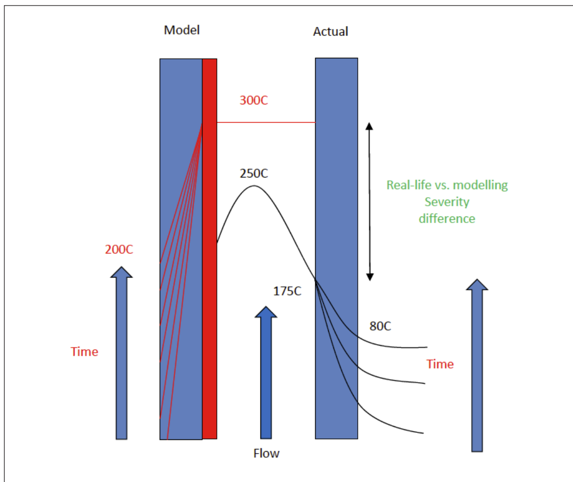
Figure 57. Comparison of inputs of historic conduction work with full-scale measurements.
